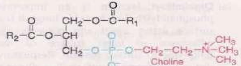
(2) Lecithin (phosphatidylcholine)
