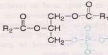
(1) Phosphatidic acid
