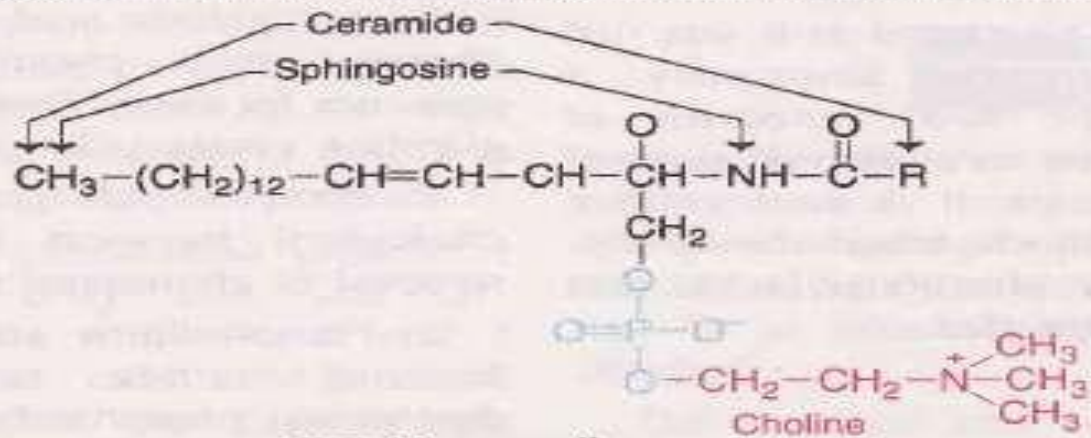
(8) Sphingomyelin
